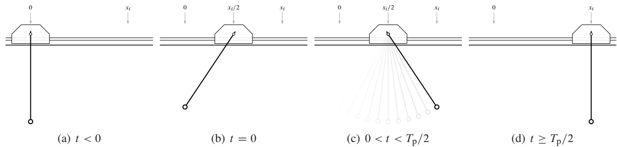
Fig. 8.1: Posicast control of a cart with a pendulum with the period T_p
