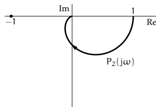
(ב) P_2(s)
