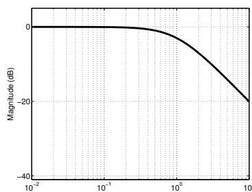
(ו) G_3(s)
