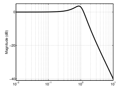
(ד) G_1(s)
