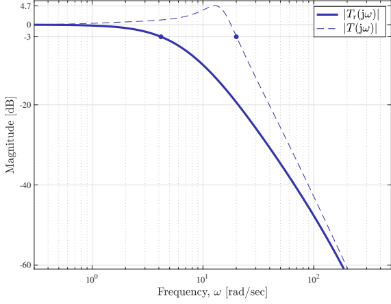
(a) Bode magnitude plot of T_{yr}(s)
