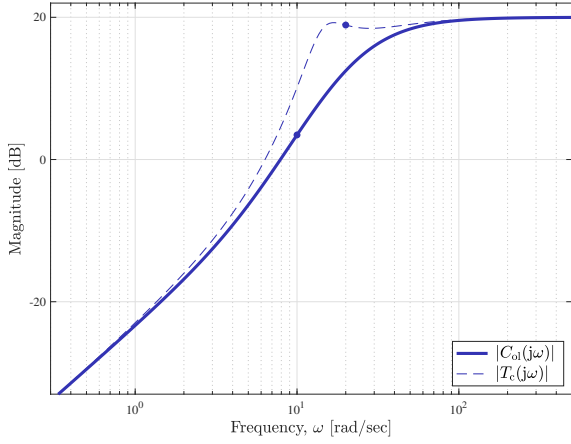
(c) Bode magnitude plot of T_{ur}(s)
