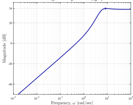
Boode magnitude plot of T_c(j\omega)
