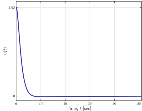
Step response of T_c(s)
