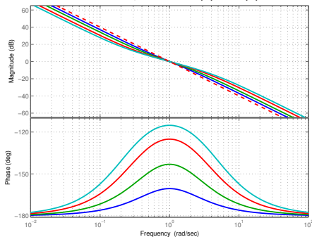
Bode diagrams of P(s)C_{\text{lead}}(s)
