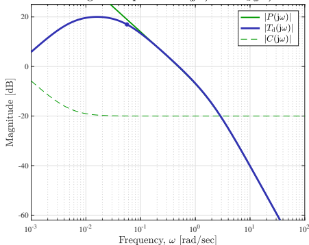
Boode magnitude plots of P(j\omega) and T_d(j\omega)
