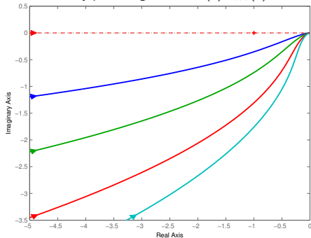
Nyquist diagrams of P(s)C_{\text{lead}}(s)
